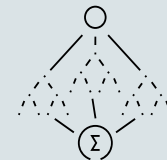
Random Forest
