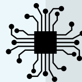
Neuronal Networks
